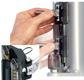
Quick-release button
