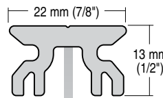
3807 Slug-mount track
